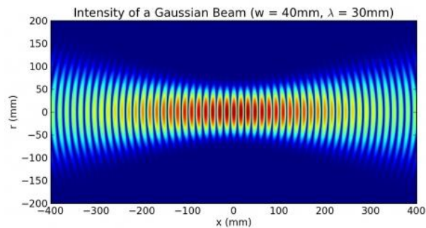
2d example of beam profile
